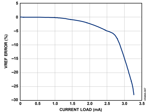
Figure 65. VREF Accuracy vs. Load
